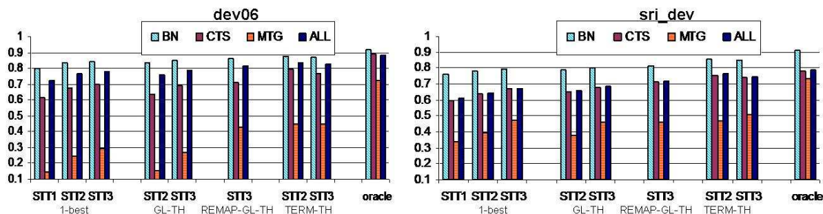
Figure 2: ATWV results on all subsets of dev06 and sri_dev using different indexing and thresholding approaches
